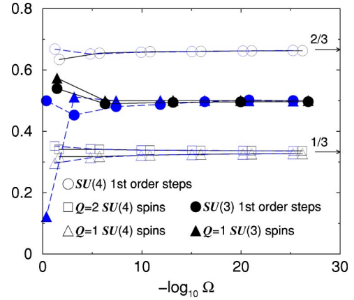
FIG. 1. (Color online) The fractions of first-order decimation steps, of spins in the fundamental ( Q=1 ), and in the self-conjugate [ Q=2 , only for SU (4)] representations, all as a function of \Omega . For clarity, we only show data for chains A (solid lines) and E (dashed lines) (see text). The filled (open) symbols refer to the SU (3) [SU (4)] chains. The data error is about the size of the symbol.
