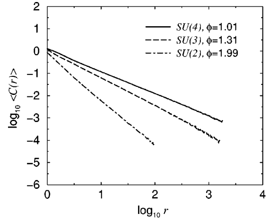
FIG. 3. Mean correlation function for groups SU (2), SU (3), and SU (4). The power-law dependence is evident. The exponents \phi=1.99\pm 0.03 , 1.31\pm 0.03 , and 1.01\pm 0.03 are obtained by fitting the region r>10 , and are in excellent agreement with the analytical value \phi=4/N [see Eq. (8)].
