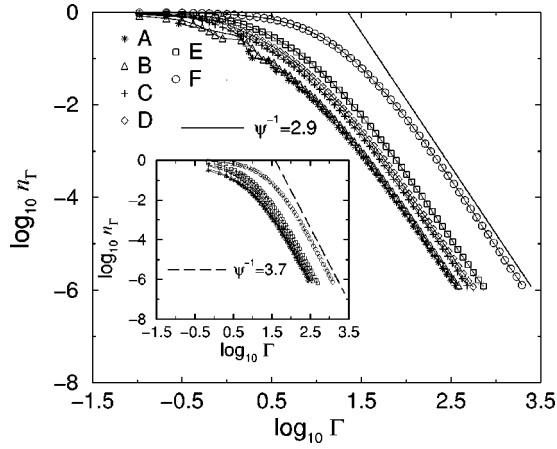
FIG. 2. Fraction of active spins n_\Gamma as a function of the energy scale \Gamma , for the SU (3) (main) and SU (4) (inset) chains A to F. The data error is smaller than the symbol size.
