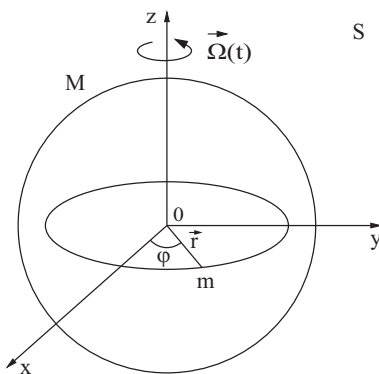
Figure 1: Spherical shell spinning around the z axis with an internal ring at the equatorial plane.
